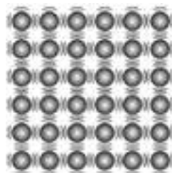
(b) Particles with increased vibrations
