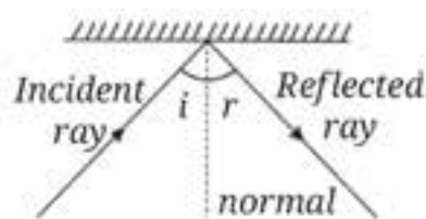
Angle of incidence and angle of reflection
