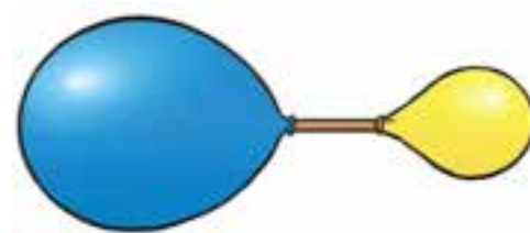
Figure 6.12: Air moves from a high pressure region to a low pressure region
