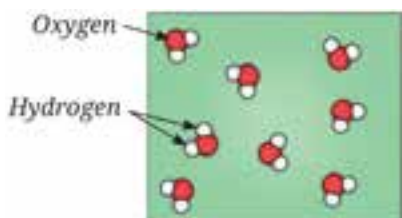
Depiction of molecules of water
