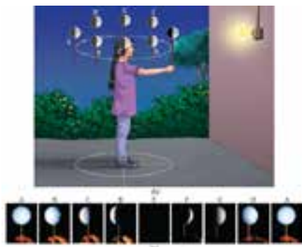
(b) A student using a ball and stick to understand phases of Moon; (c) The ball as seen by the student at different positions
