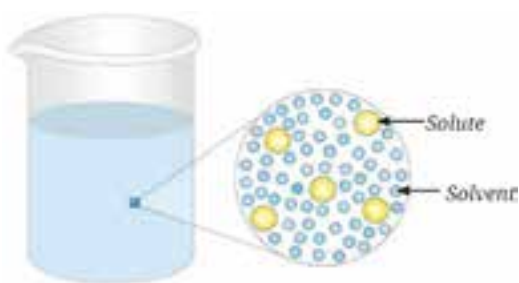
Magnified schematic picture of a solute evenly distributed in a solvent
