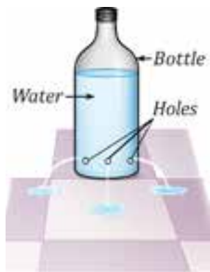
Liquid exerts pressure on the wall of the container
