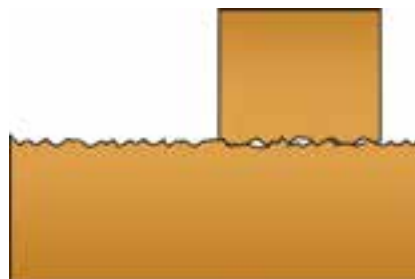
Friction between two surfaces due to irregularities
